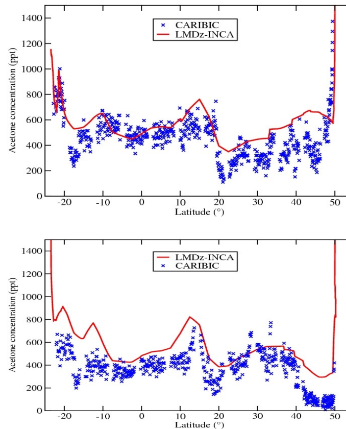
•Figure 2. Acetone concentrations are plotted as a function of the latitude during the CARIBIC Frankfurt-Sao Paulo (a) and back (b) of 20-21 March 2006. Measurements within the CARIBIC experiment (blue cross) are compared to 30-minute resolution simulations generated by the LMDz-INCA model (red line).
